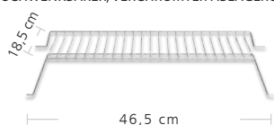
MASSIVE GUSSROSTE
